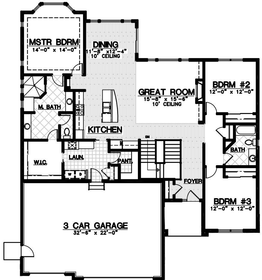
MAIN LEVEL PLAN
