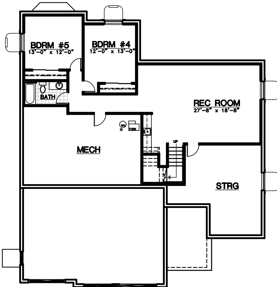
LOWER LEVEL PLAN OPTIONAL FINISHED
